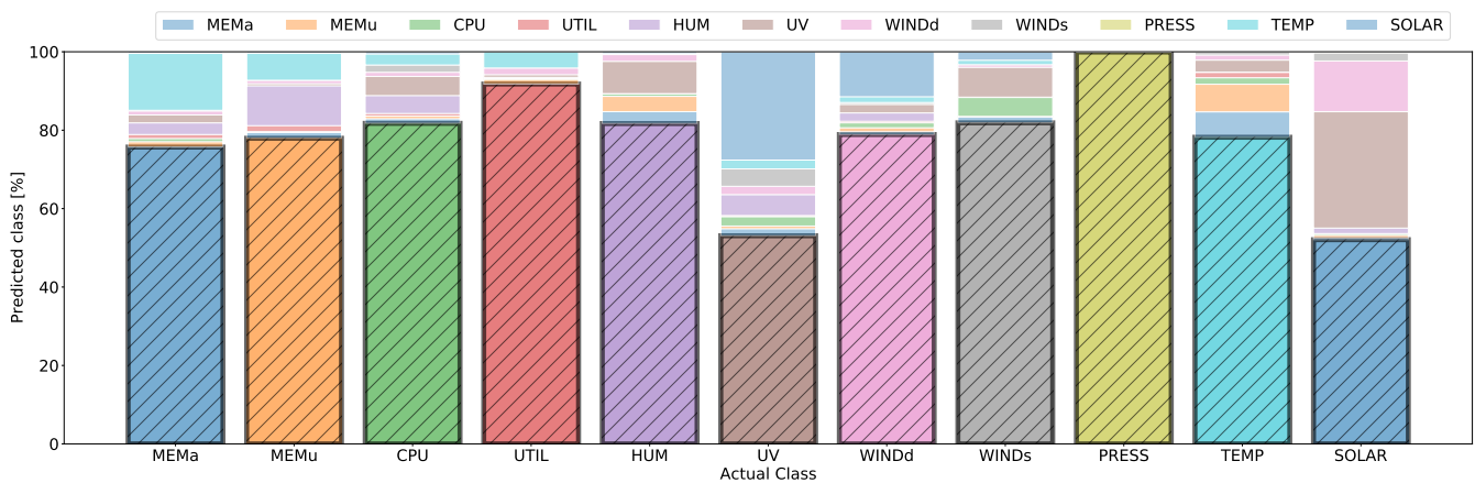
Figure 6.12. Accuracy of mc RF streaming data
