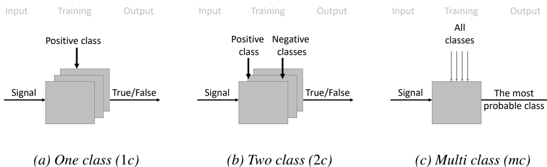
Figure 6.2. Illustration of three approaches
