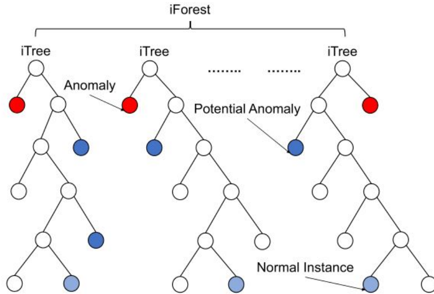
Figure 3.10. Isolation forest [7]
