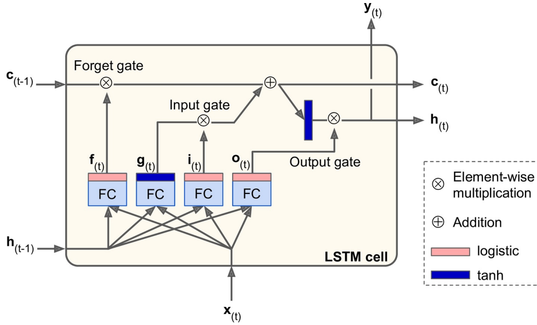
Figure 3.7. Long short-term memory (LSTM) cell [4]
