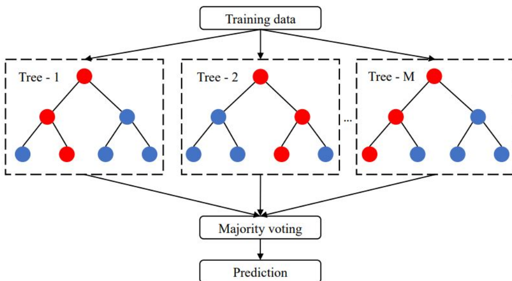
Figure 3.2. Illustration of random forest [2]
