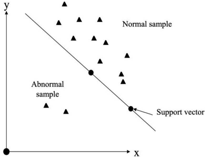
Figure 3.9. One class support vector machine [6]
