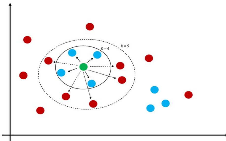
Figure 3.4. Illustration of an example of the k -nearest neighbor algorithm [3]
