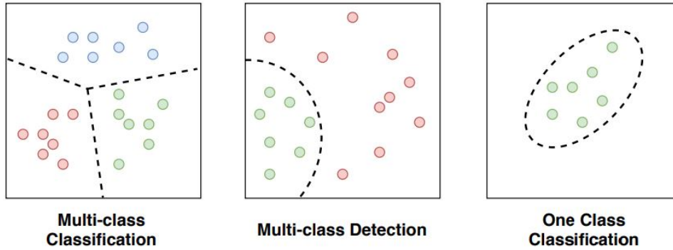
Figure 3.8. One class classification vs multi-class classification/detection [5]
