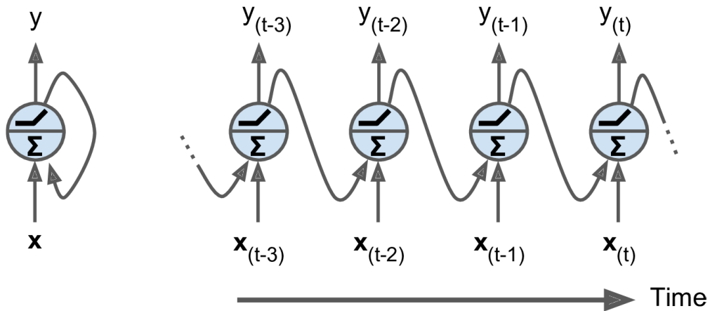
Figure 3.6. A recurrent neuron [4]
