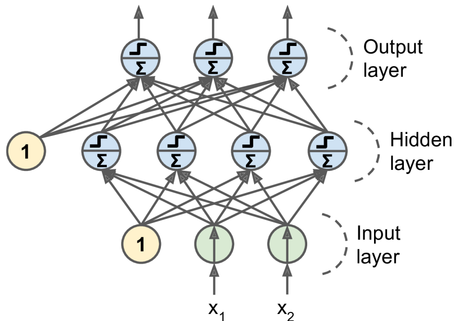
Figure 3.5. Multilayer Perceptron [4]
