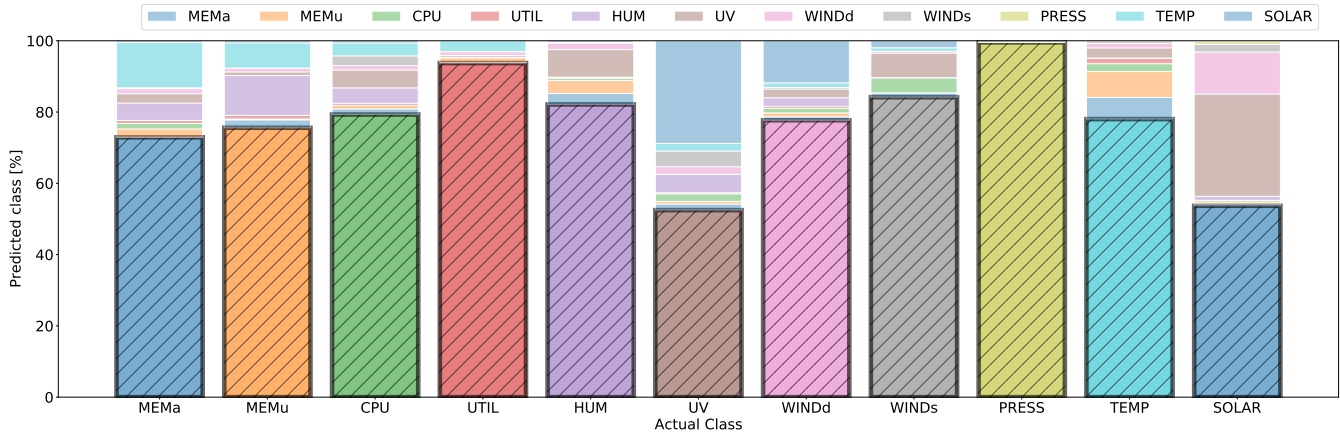
Figure 6.14. Accuracy of mc RF stored data
